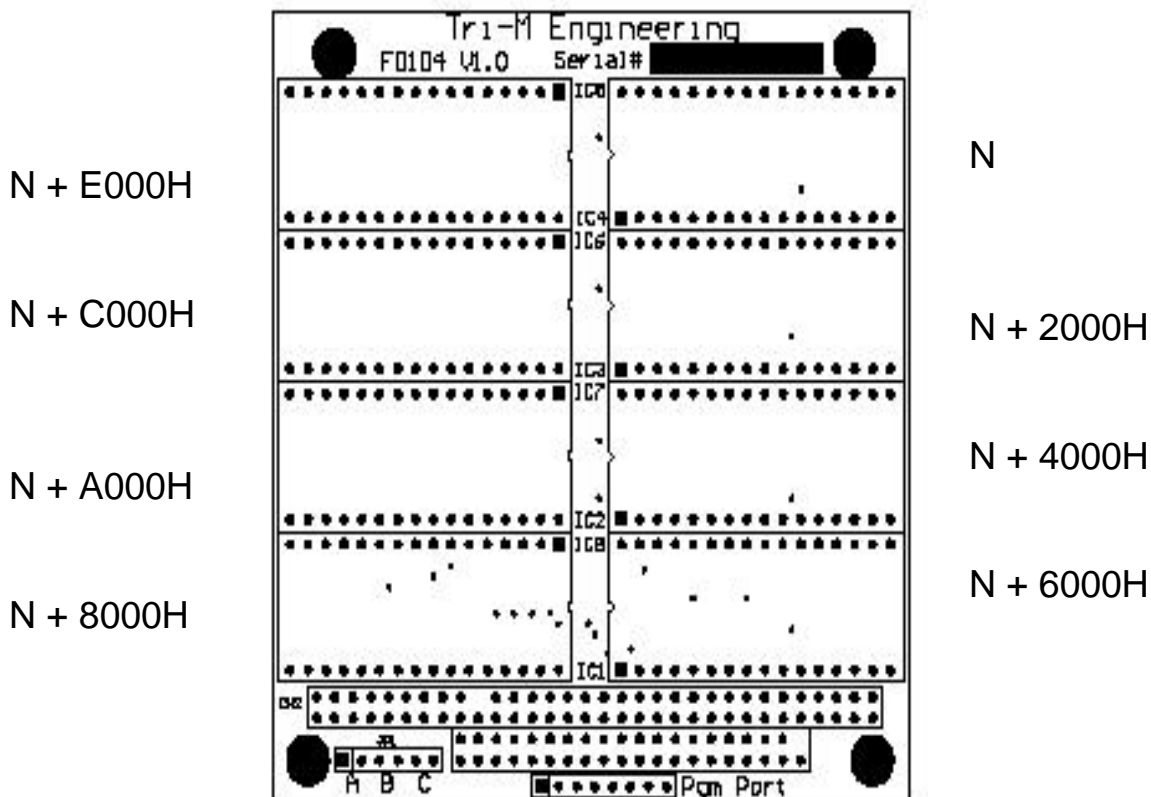
Figure 2. MD104 socket address
