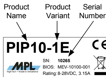
Figure 17: PIP10-E Label
