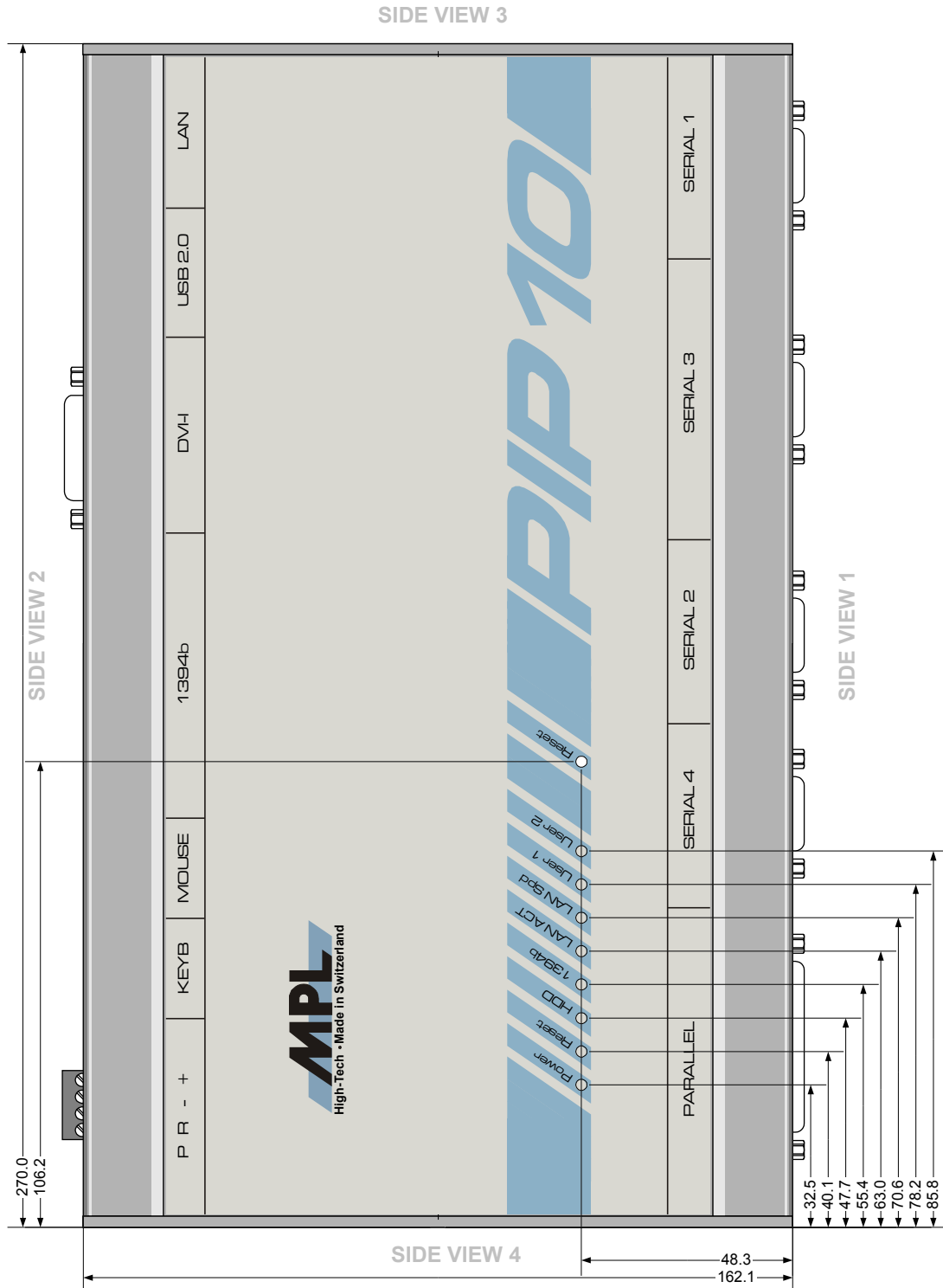
Figure 1: PIP Housing Top View
