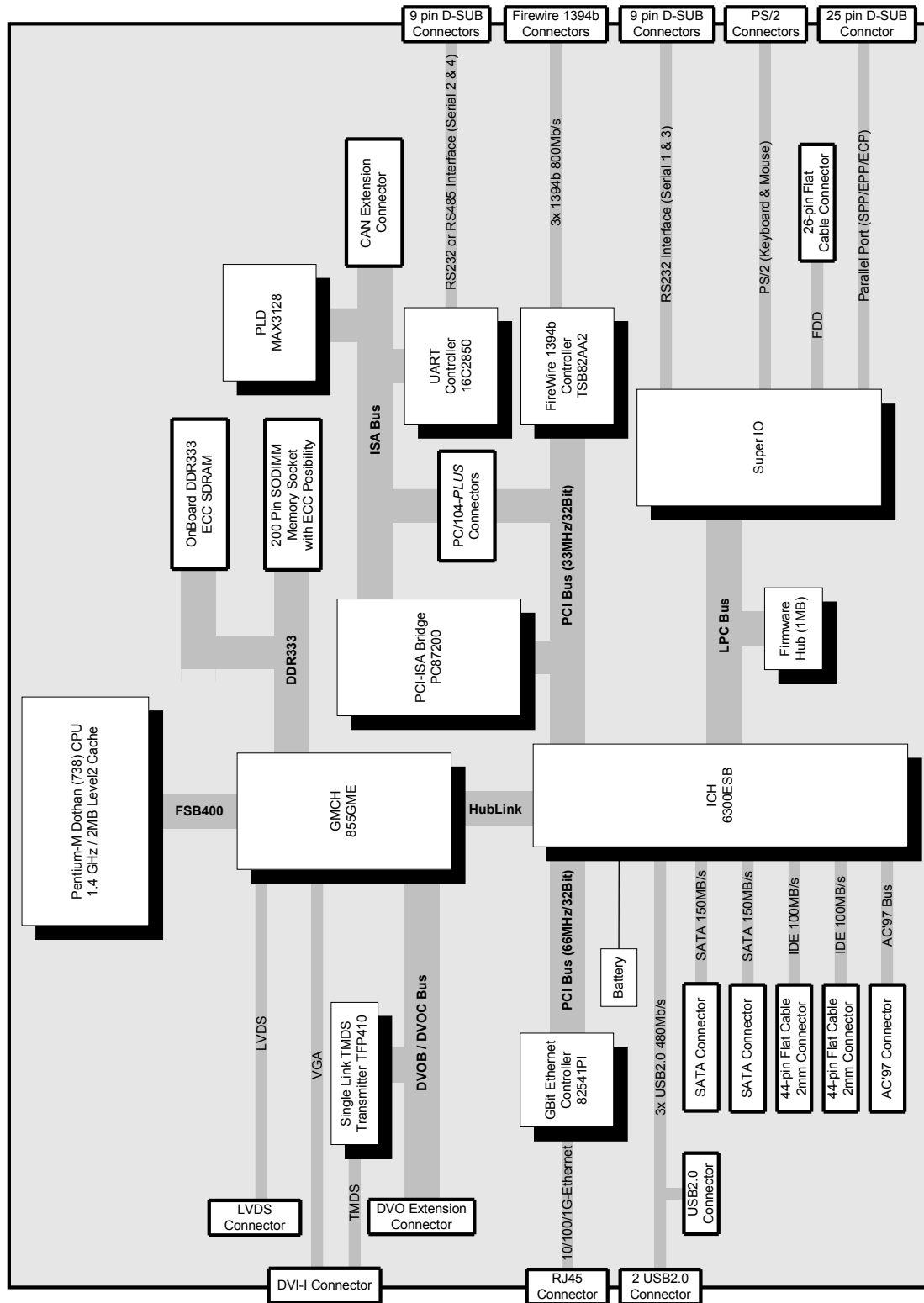
Figure 17: PIP10-1 Block Diagram
