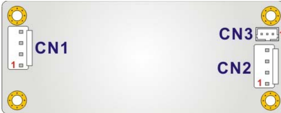
Figure 2: IDD-241100/481100 Connector and Jumper Locations
