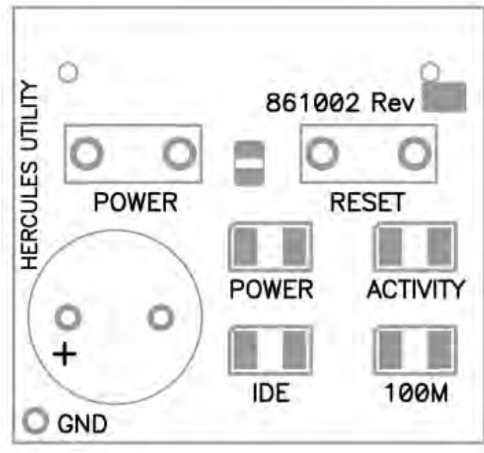
Figure 44: Utility Board
