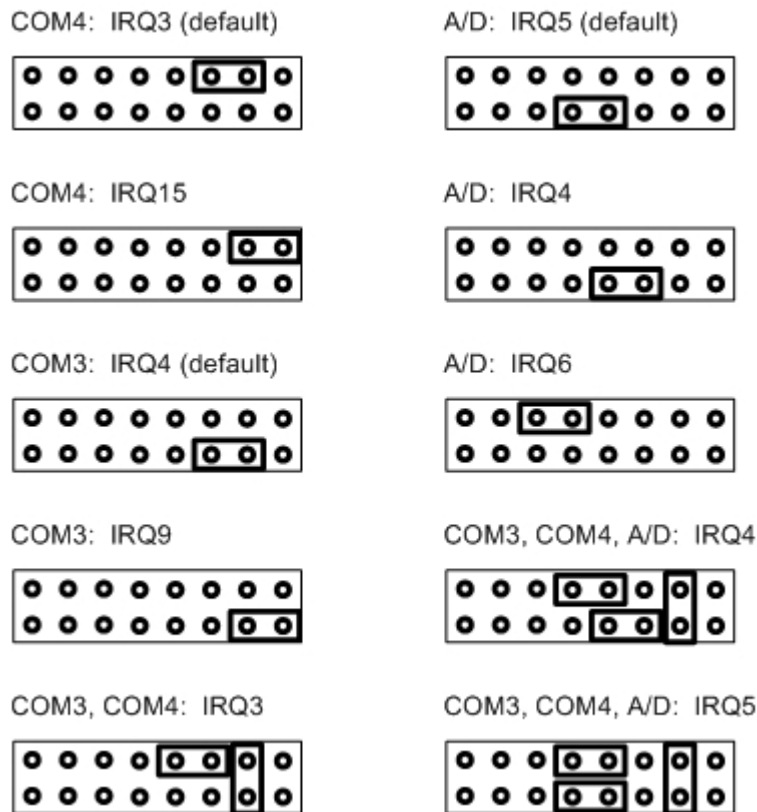
Figure 22: IRQ Configuration Options
