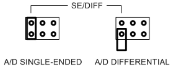
Figure 26: A/D Single-ended/Differential Selection
