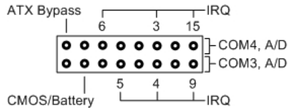
Figure 21: J10 Jumper Block
