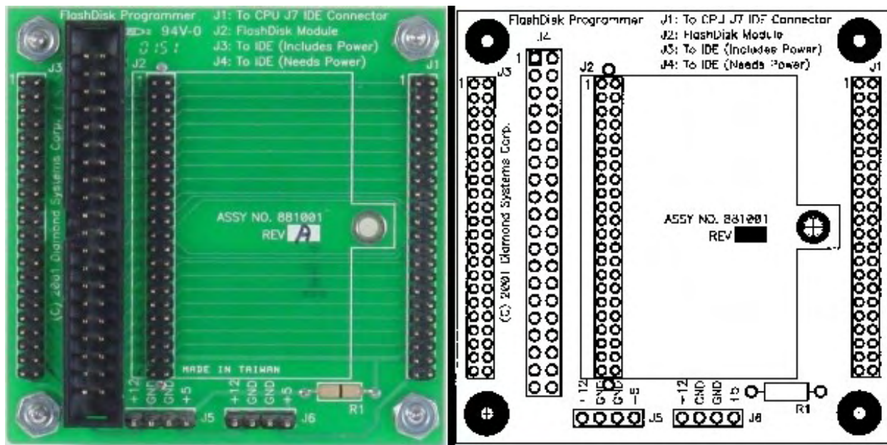
Figure 32: FlashDisk Programmer Board Layout
