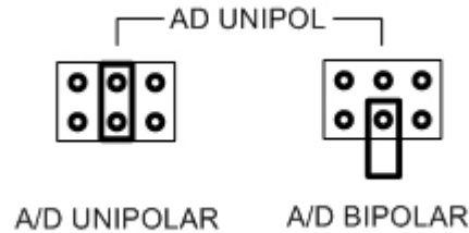
Figure 27: A/D Unipolar/Bipolar Selection
