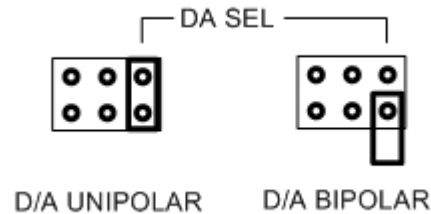
Figure 28: Analog Output Configuration Selection
