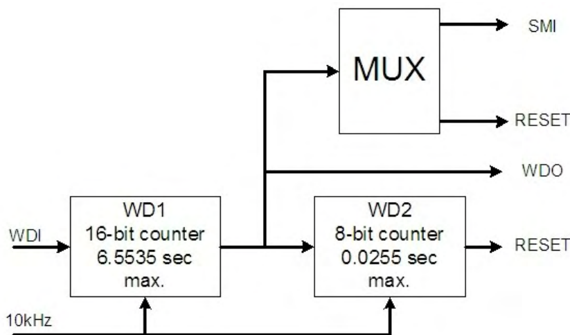
Figure 29: Watchdog Timer Block Diagram
