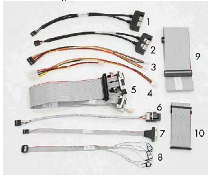
Figure 33: Cable Kit C-ATH-KIT
