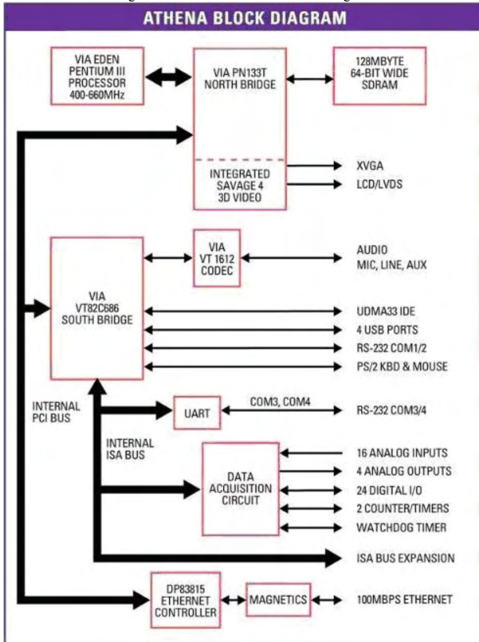
Figure 1: Athena II Functional Block Diagram
