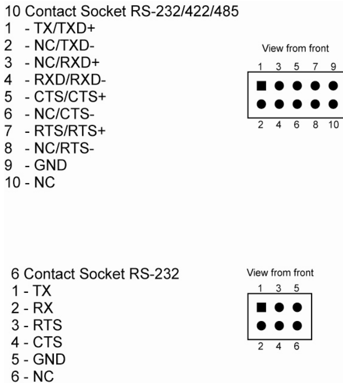
Figure 7: Pinouts
