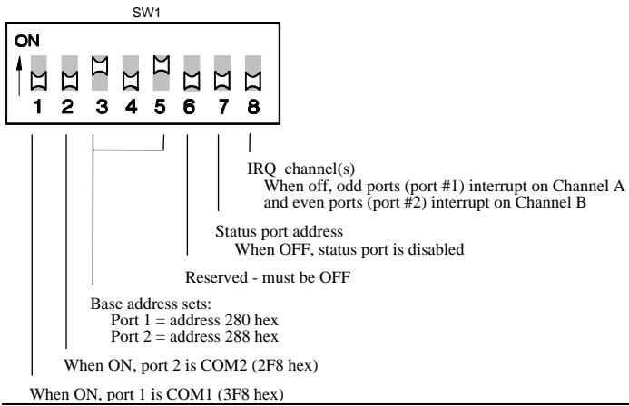
Figure 21: Windows 3.XX: switch settings
