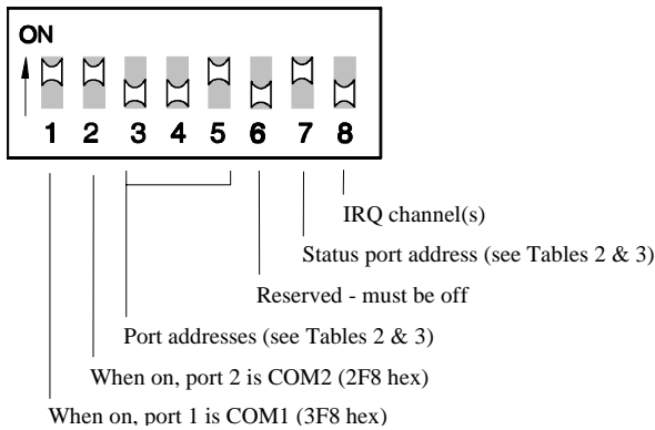
Figure 6: DIP switch block SW1
