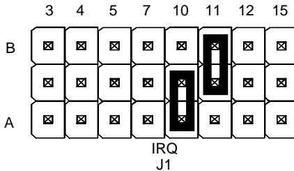
Figure 12: OS/2: IRQ settings - J1
