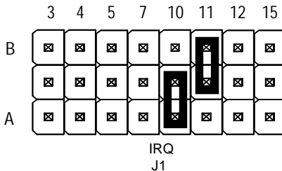
Figure 22: Windows 3.XX: IRQ settings
