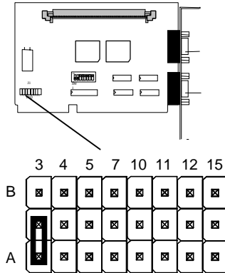
Figure 29: DFlex-2/-2/Fast: J1 factory setting
