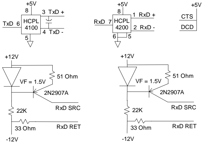
Figure 43: 20mA Current Loop schematic
