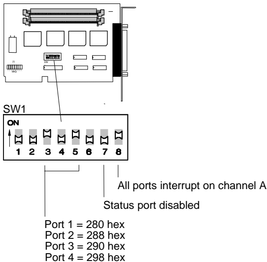
Figure 30: DFlex-4/-4/Fast: SW1 factory settings
