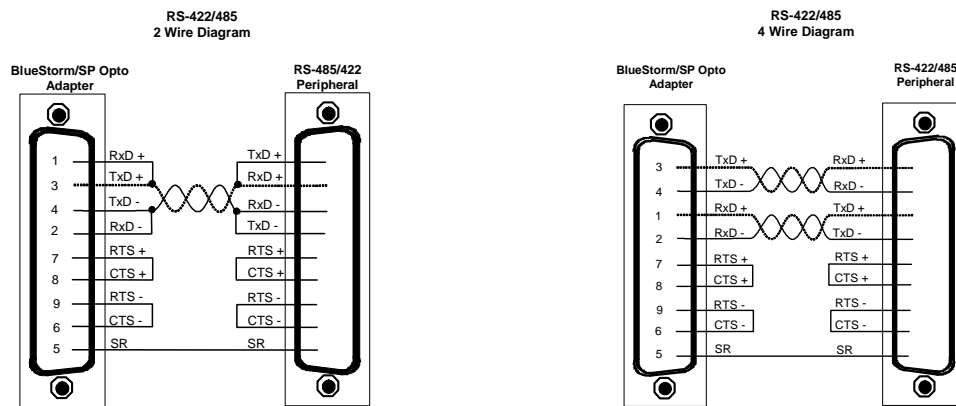
Figure 9: RS-422/485 Wiring Diagrams (BlueStorm/SP Opto only)
