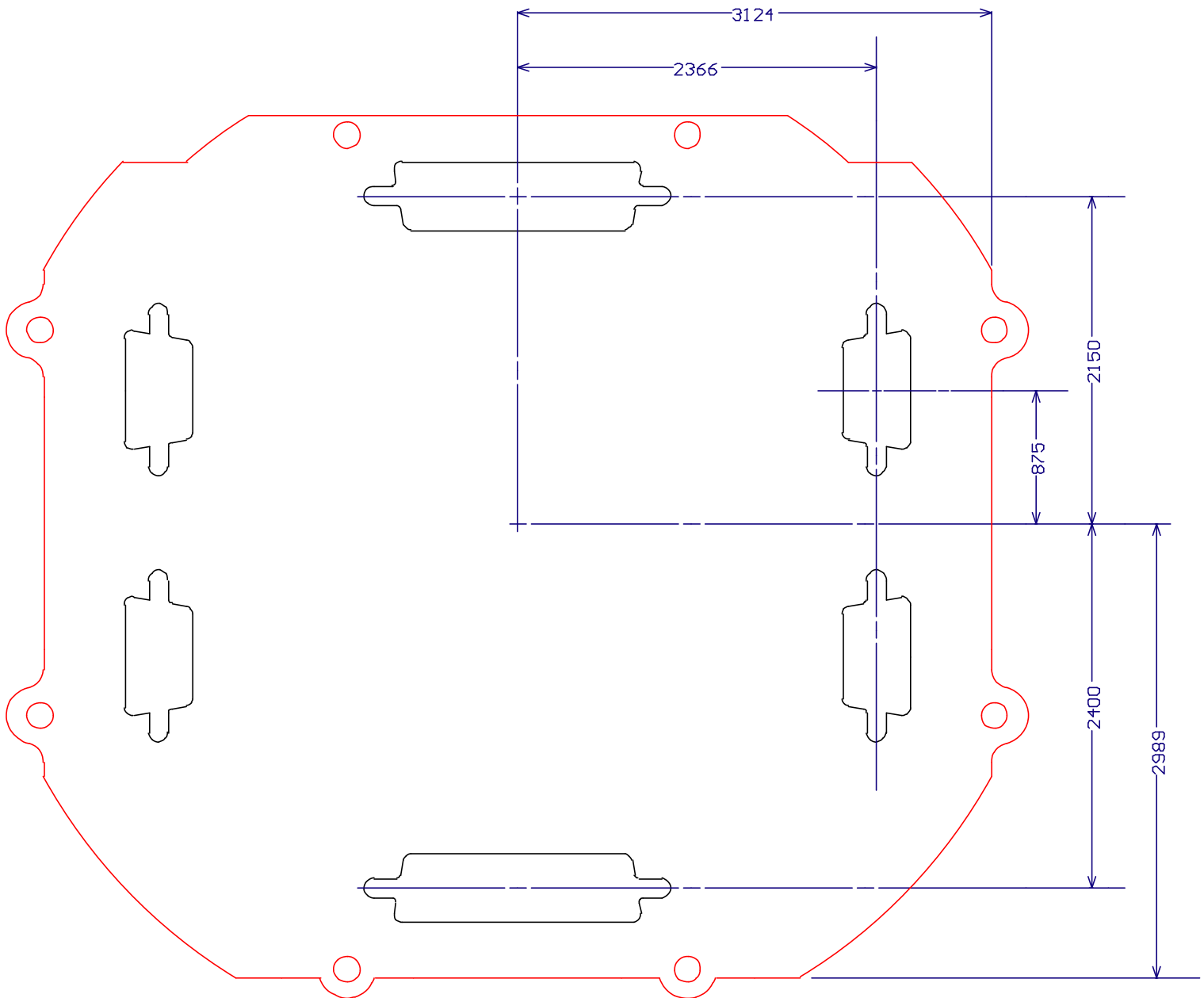
VersaTainer VT-EC02 Layout Tri-M Engineering www.Tri-M.com
